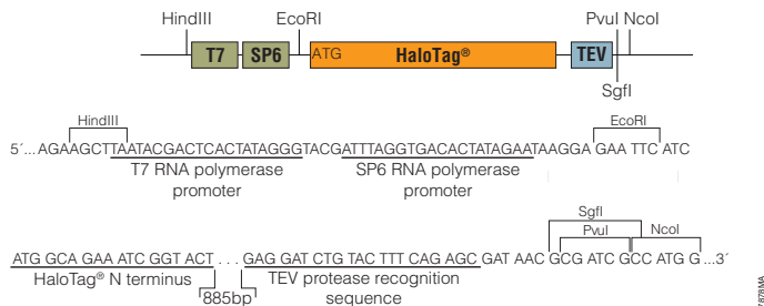
Figure 2. pFN23K HaloTag® CMVd2 Flexi® Vector sequence upstream and downstream of the HaloTag® gene.
