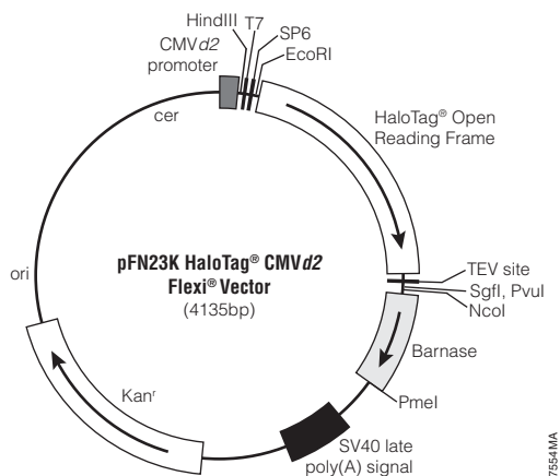
Figure 1. pFN23K HaloTag® CMVd2 Flexi® Vector circle map and sequence reference points.
